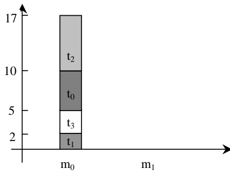
Figure 3. the Min-min gives a makespan of 17
