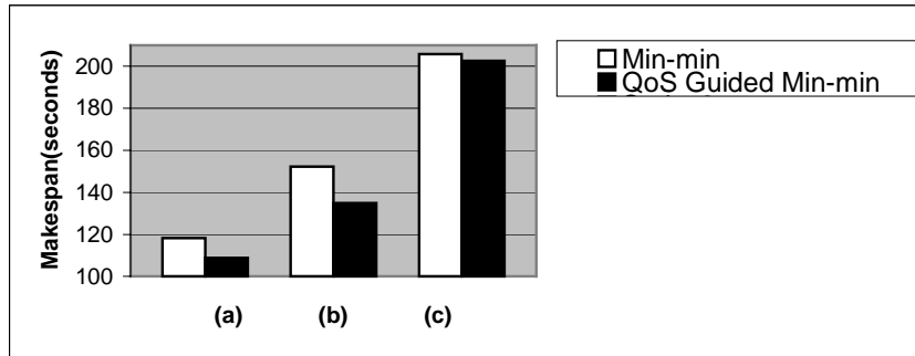
Figure 5. Makespan for three scenarios for two heuristics
